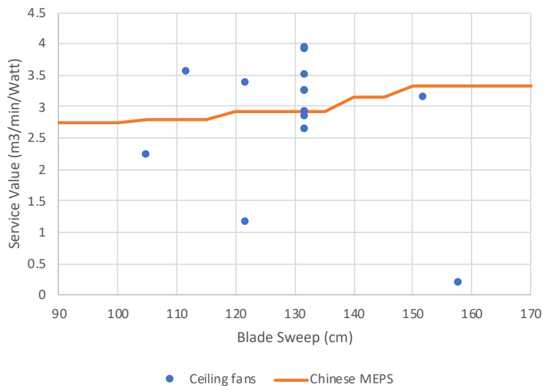
Figure 9: Comparison of ceiling comfort fans with the Chinese MEPS (data gathered by Topten, 2018).
