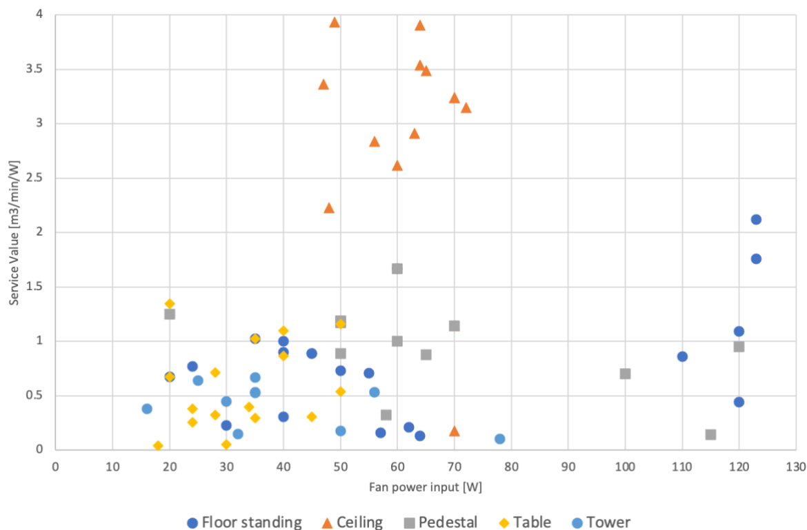
Figure 6: Distribution of fans (according to construction types) in relation to the Service Value. The Topten selection criteria were based on the service value and selected the 50% best performing products (data gathered by Topten, 2018).
