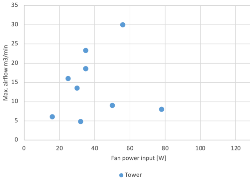
Figure 5: Distribution of tower comfort fans according to maximum airflow [m 3 /min] and fan power input [W] (data gathered by Topten, 2018)
