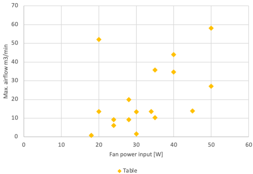
Figure 4: Distribution of table comfort fans according to maximum airflow [m 3 /min] and fan power input [W] (data gathered by Topten, 2018)
