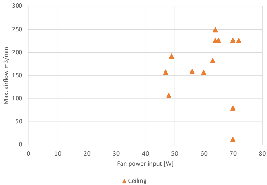
Figure 2: Distribution of ceiling comfort fans according to maximum airflow [m 3 /min] and fan power input [W] (data gathered by Topten, 2018)
