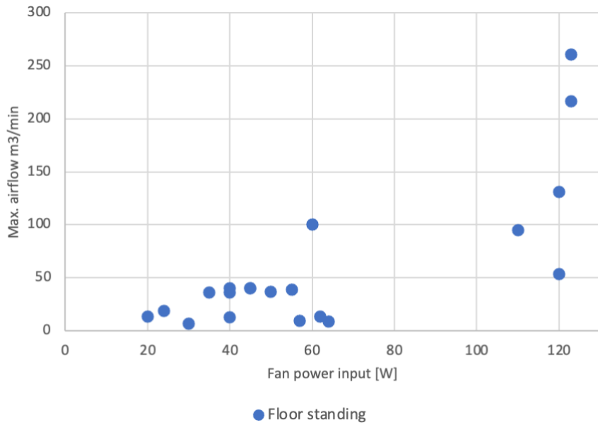
Figure 1: Distribution of floor standing comfort fans according to maximum airflow [m 3 /min] and fan power input [W] (data gathered by Topten, 2018)
