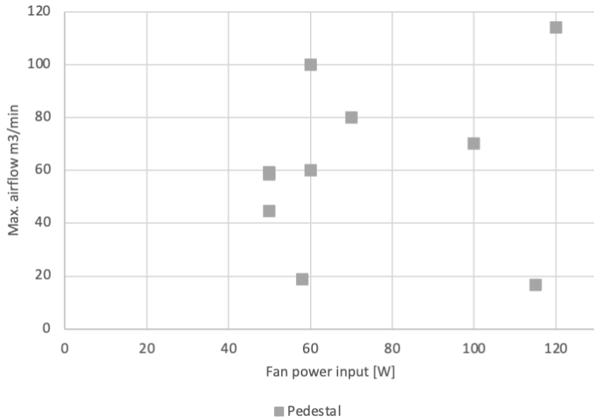
Figure 3: Distribution of pedestal comfort fans according to maximum airflow [m 3 /min] and fan power input [W] (data gathered by Topten, 2018)
