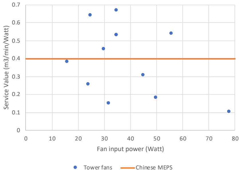
Figure 8: Comparison tower comfort fans with the Chinese MEPS (data gathered by Topten, 2018).
