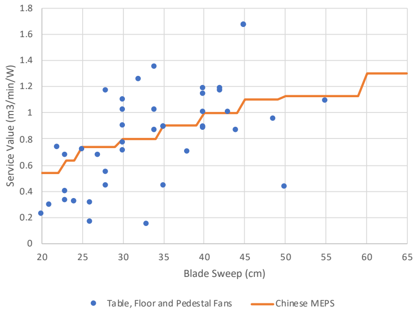
Figure 7: Comparison of table, floor, and pedestal comfort fans with the Chinese MEPS (data gathered by Topten, 2018).
