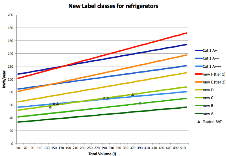
Figure 2: Current and new proposed classes for refrigerators. With Ecodesign tiers and Topten Best Available Technologies (BAT). Source: Topten, own calculations, 2018.
