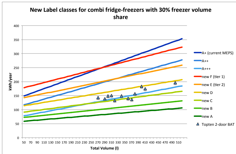
Figure 3: Current and new proposed classes with Ecodesign tiers. Neither compensation factors nor the possible effects of the new measurement standard have been considered in this chart. Source: Topten, own calculations, 2018.
